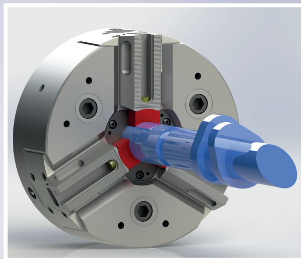
shaft clamping
