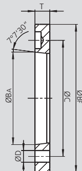
Type FF 1 ISO-A mounting direct
