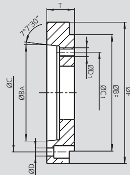
Type FF 3 ISO-A mounting increase
