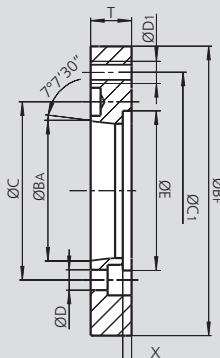
Type FF 2 ISO-A mounting reduction
