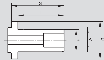
Mounting shank type ZV
