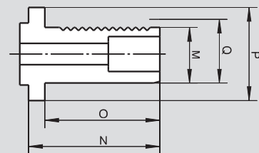
Mounting shank type ZV
