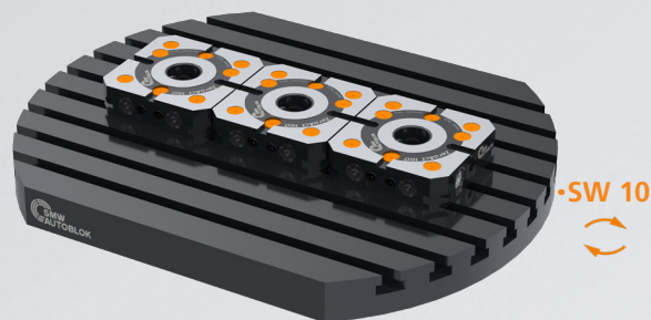
3 ZeroAct clamping modules in series
