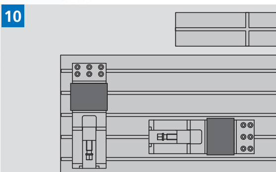
Precise T-slots for the assembling on the machine table by using positioning keys
