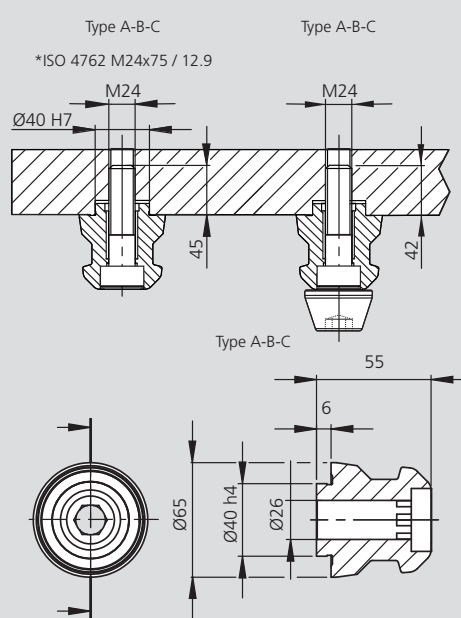
Clamping pin Ø26
