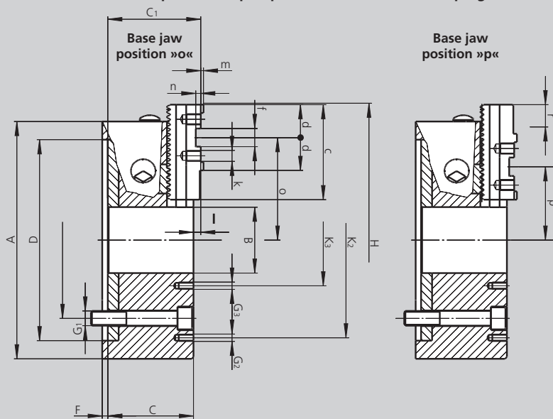
Jaw position: Open position for external clamping
