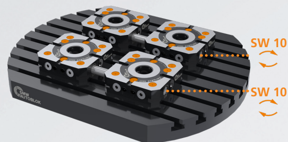
4 ZeroAct clamping modules in series
